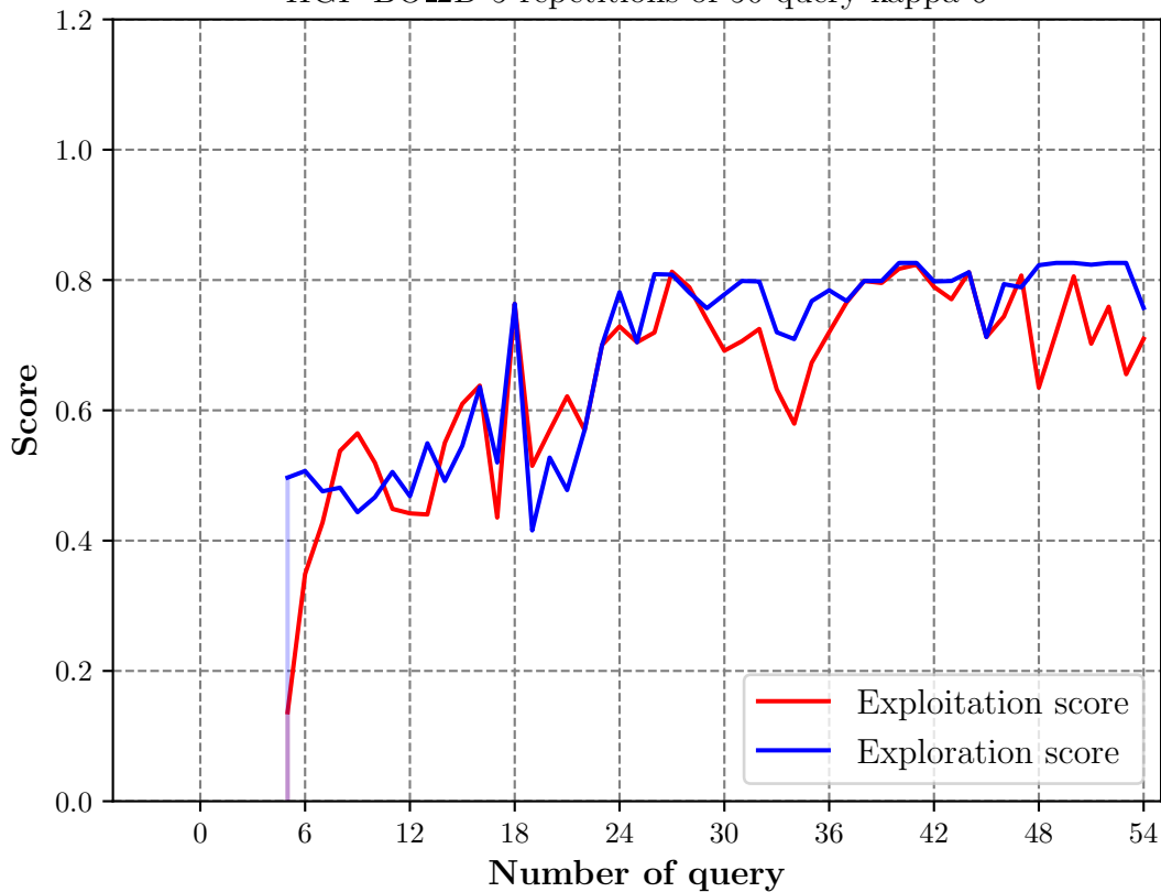
HGP-BO_2D 5 repetitions of 50 query kappa 6
